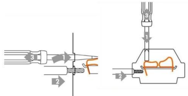
Screwless connection technology „Cage Clamp®“ (In front or on top)
